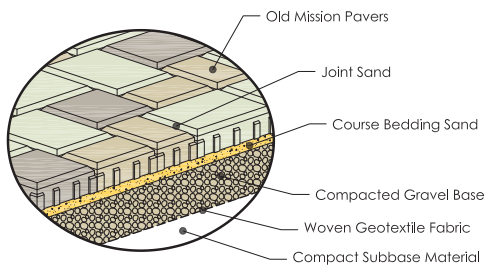
TYPICAL PAVER CROSS-SECTION
