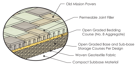
PERMEABLE PAVER CROSS-SECTION
